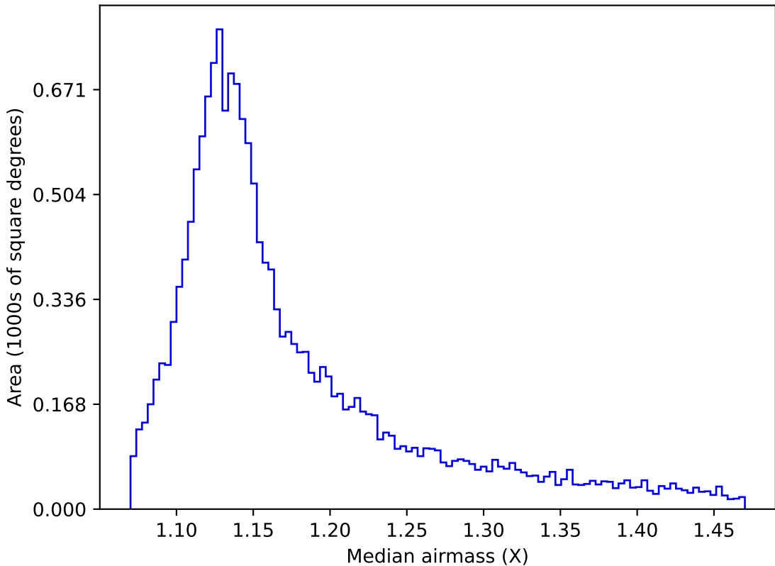
too_elab_r32_d2_gz_v3.4_10yrs WFD u band: Median airmass
