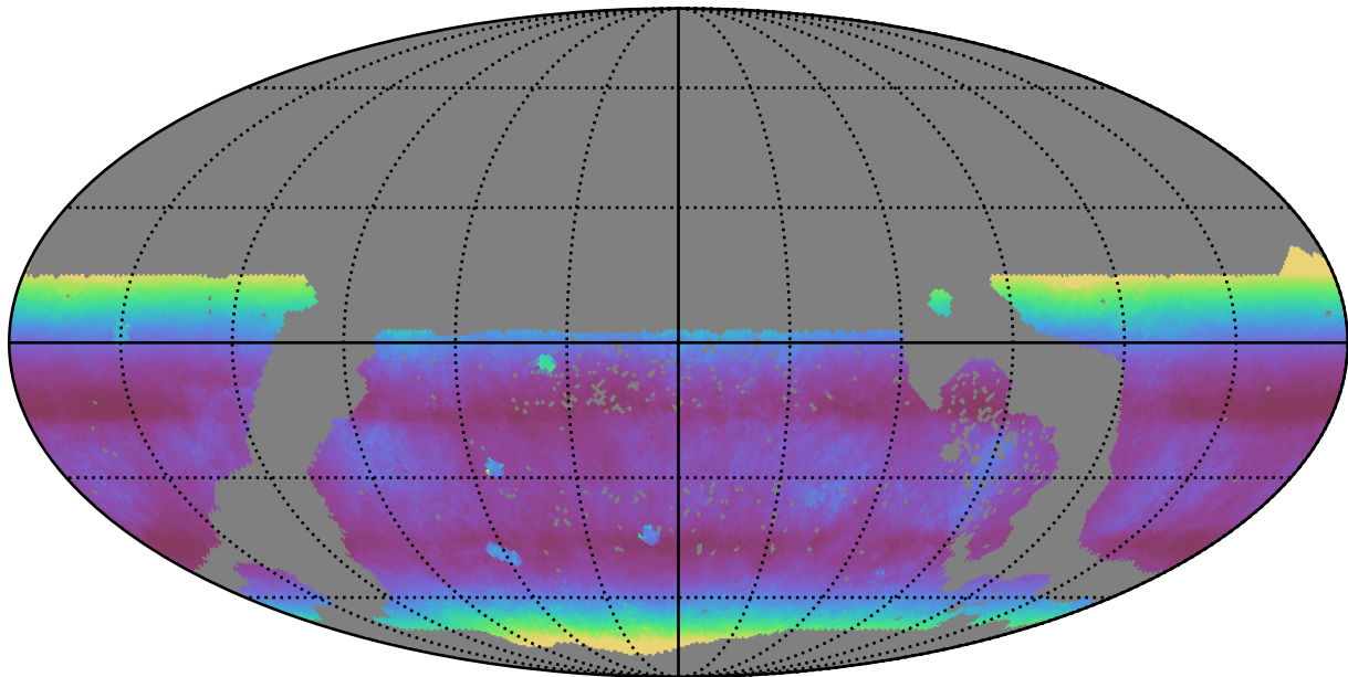
too_elab_r32_d2_gz_v3.4_10yrs WFD r band: Median airmass
