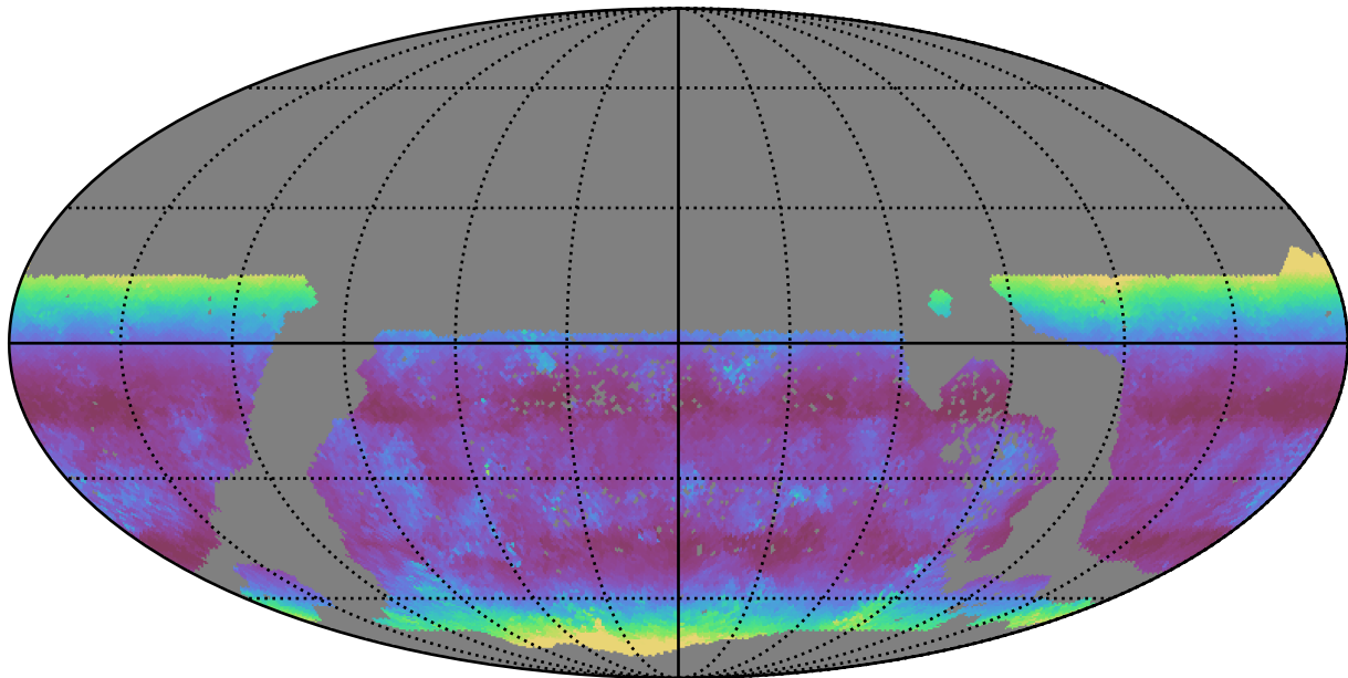
too_elab_r32_d2_gz_v3.4_10yrs WFD g band: Median airmass
