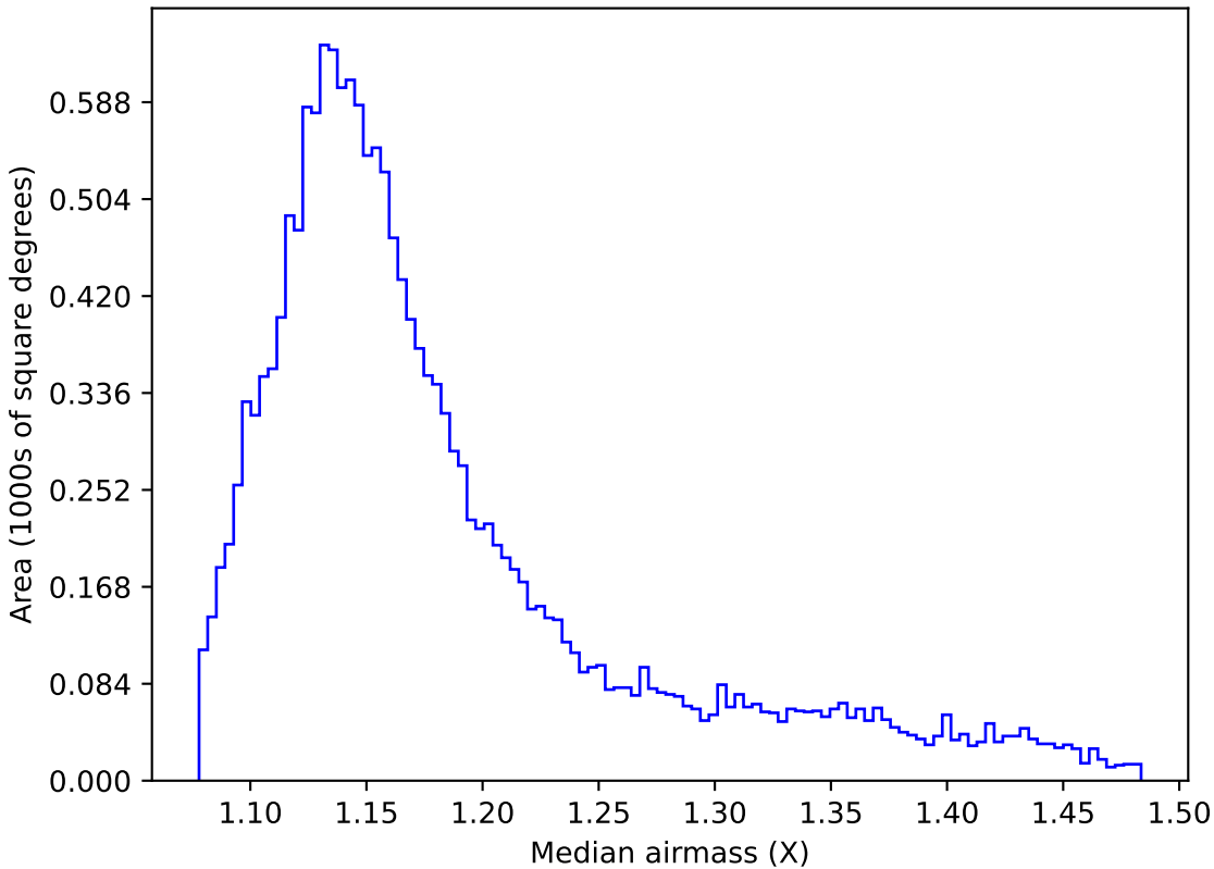
too_elab_r32_d2_gz_v3.4_10yrs WFD g band: Median airmass
