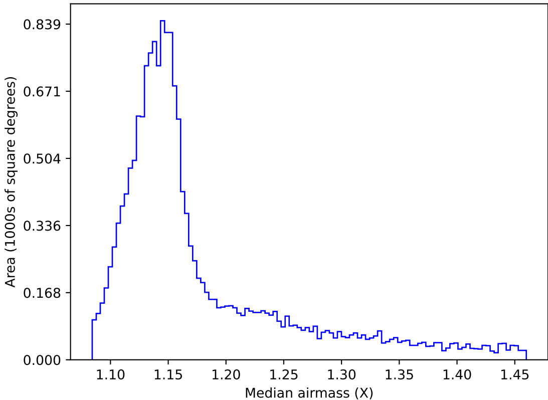
too_elab_r32_d2_gz_v3.4_10yrs WFD all bands: Median airmass
