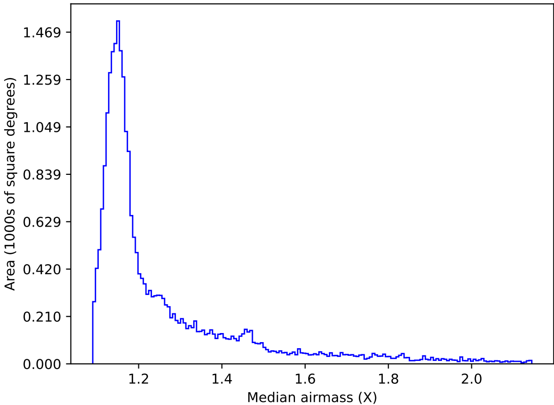
too_elab_r32_d2_gz_v3.4_10yrs All sky z band: Median airmass
