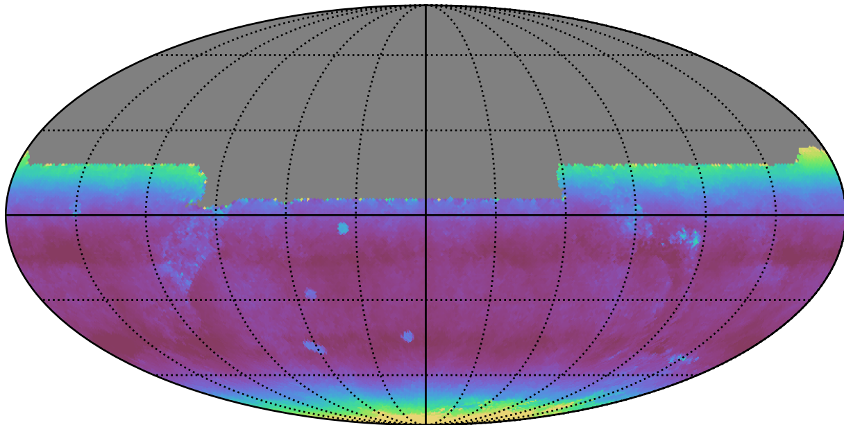
too_elab_r32_d2_gz_v3.4_10yrs All sky y band: Median airmass
