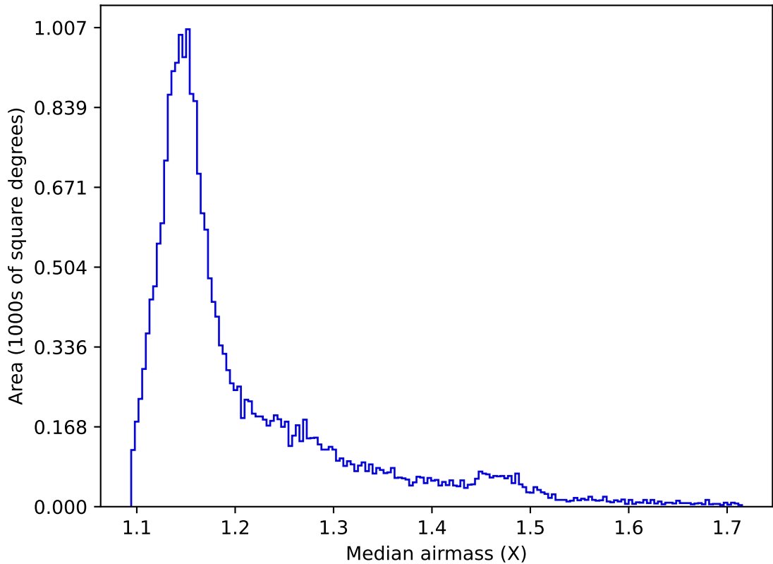
too_elab_r32_d2_gz_v3.4_10yrs All sky y band: Median airmass
