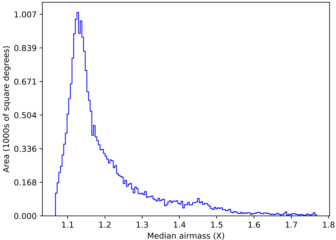
too_elab_r32_d2_gz_v3.4_10yrs All sky u band: Median airmass
