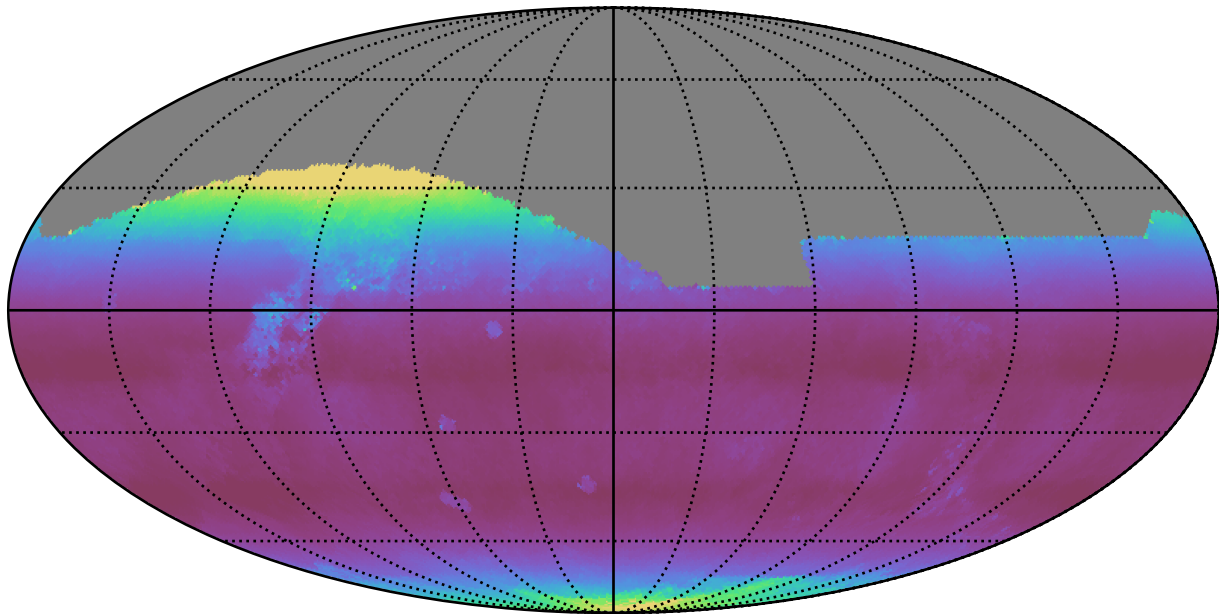
too_elab_r32_d2_gz_v3.4_10yrs All sky r band: Median airmass
