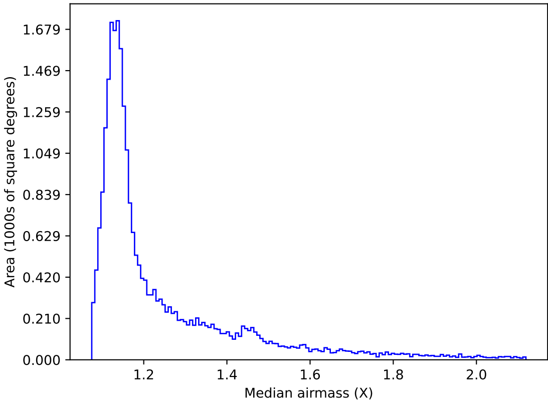
too_elab_r32_d2_gz_v3.4_10yrs All sky r band: Median airmass
