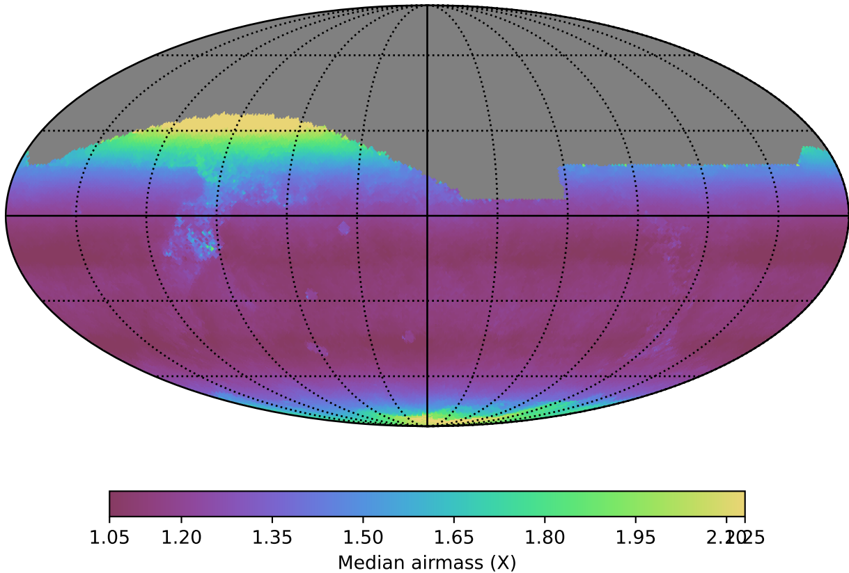
too_elab_r32_d2_gz_v3.4_10yrs All sky i band: Median airmass
