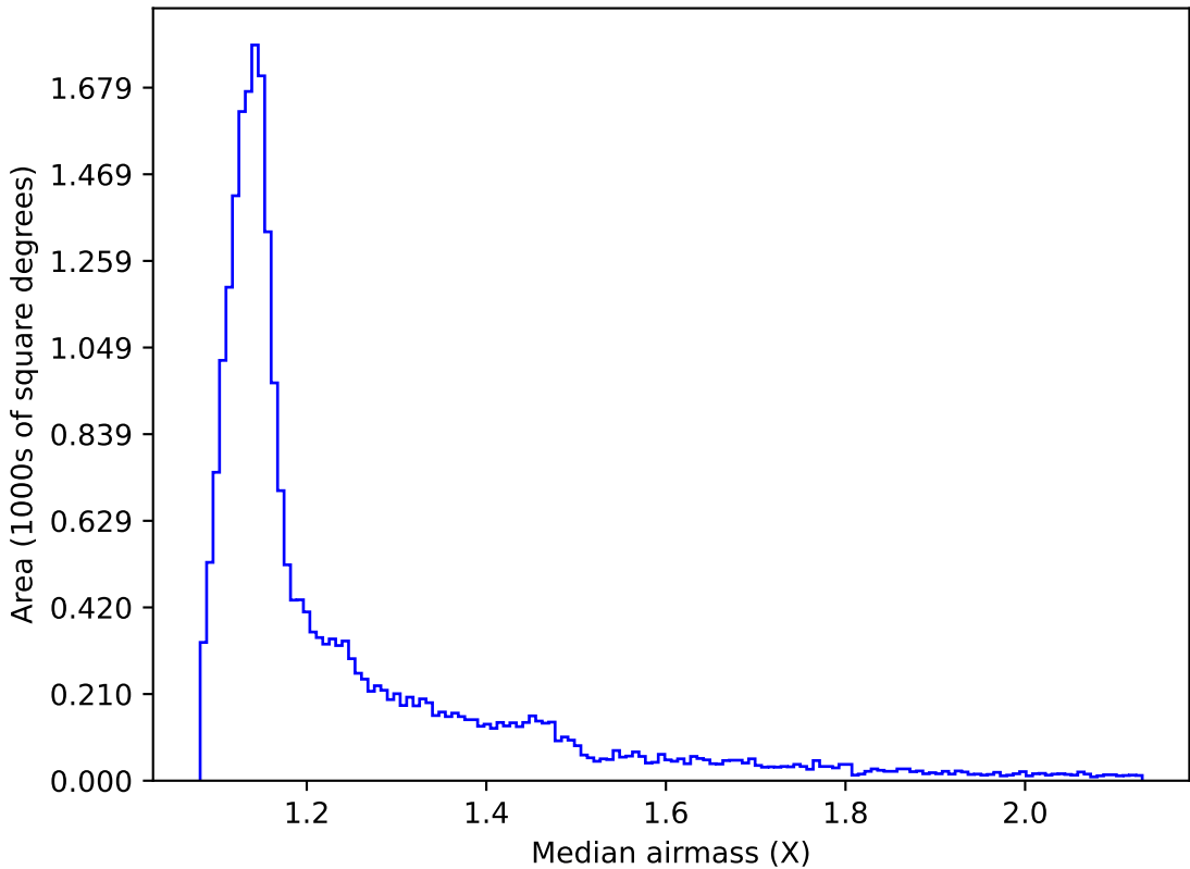
too_elab_r32_d2_gz_v3.4_10yrs All sky i band: Median airmass
