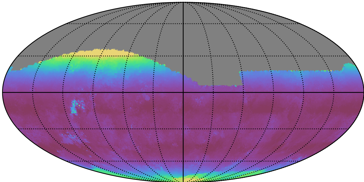
too_elab_r32_d2_gz_v3.4_10yrs All sky g band: Median airmass
