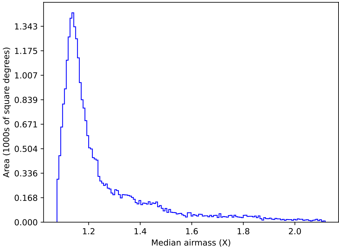
too_elab_r32_d2_gz_v3.4_10yrs All sky g band: Median airmass
