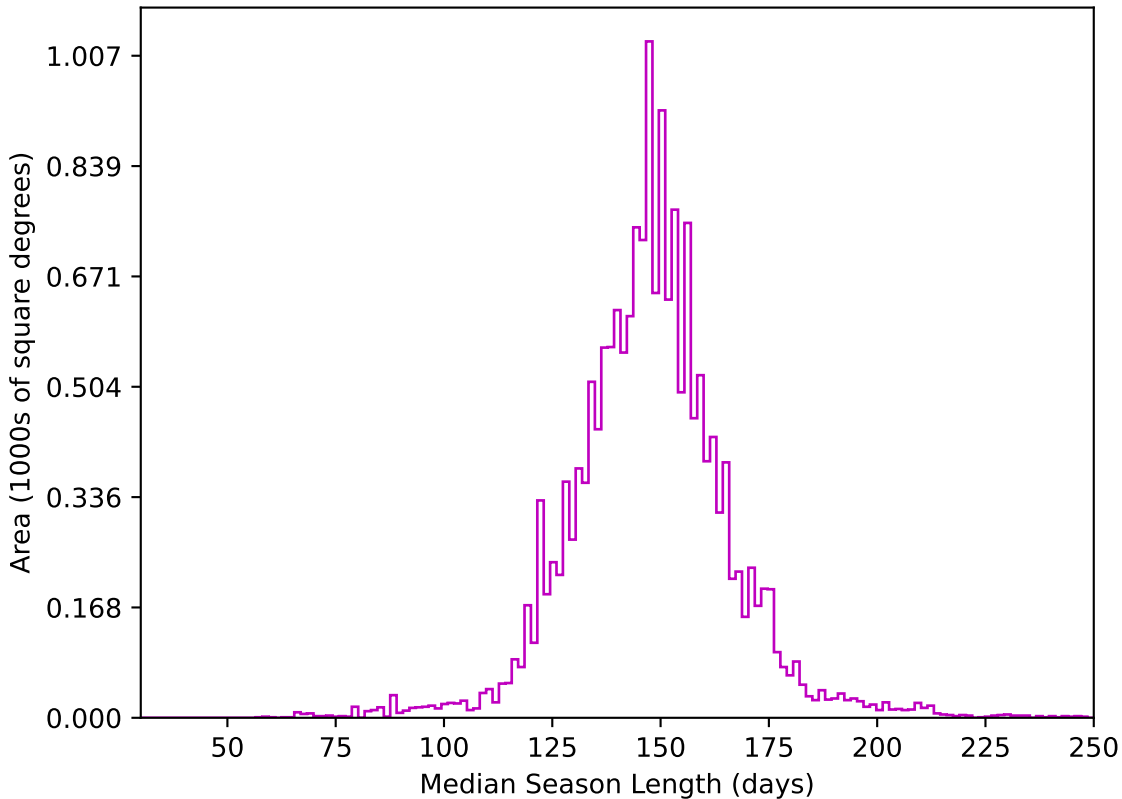
too_elab_r32_d2_gz_v3.4_10yrs WFD z band: Median Season Length
