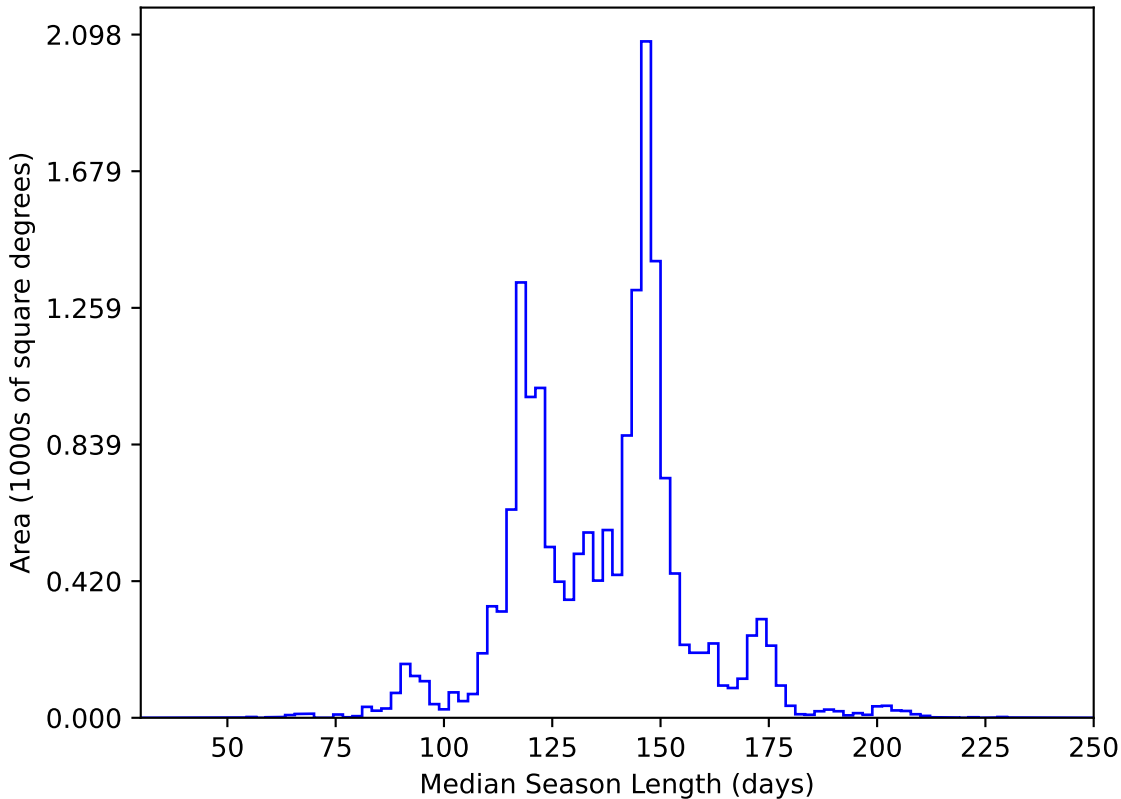
too_elab_r32_d2_gz_v3.4_10yrs WFD y band: Median Season Length
