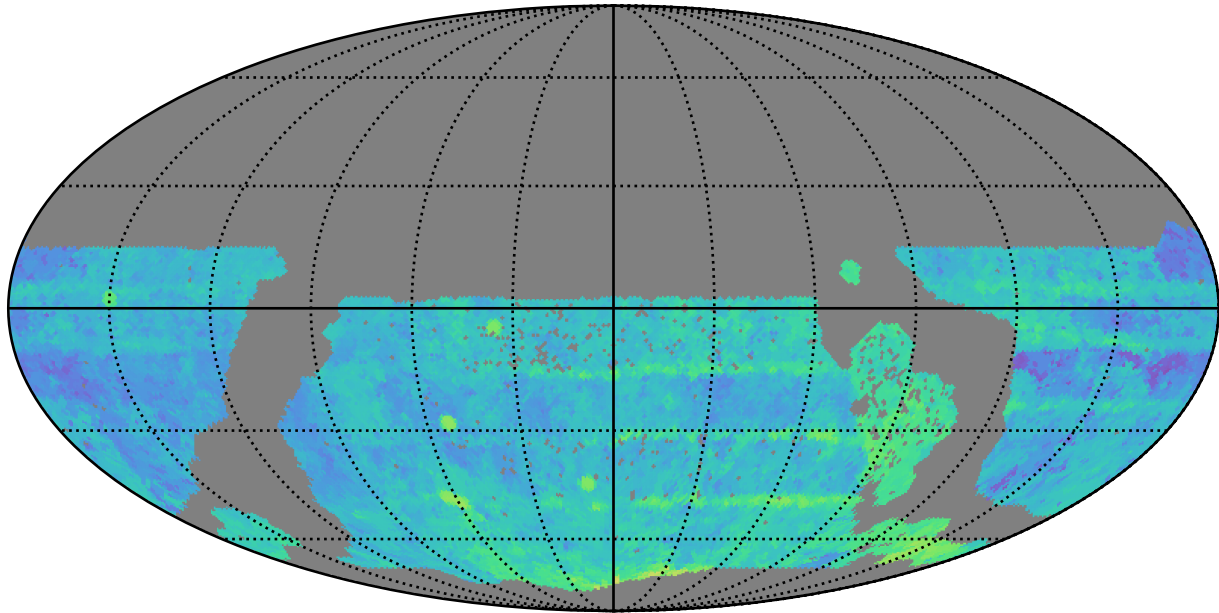
too_elab_r32_d2_gz_v3.4_10yrs WFD r band: Median Season Length
