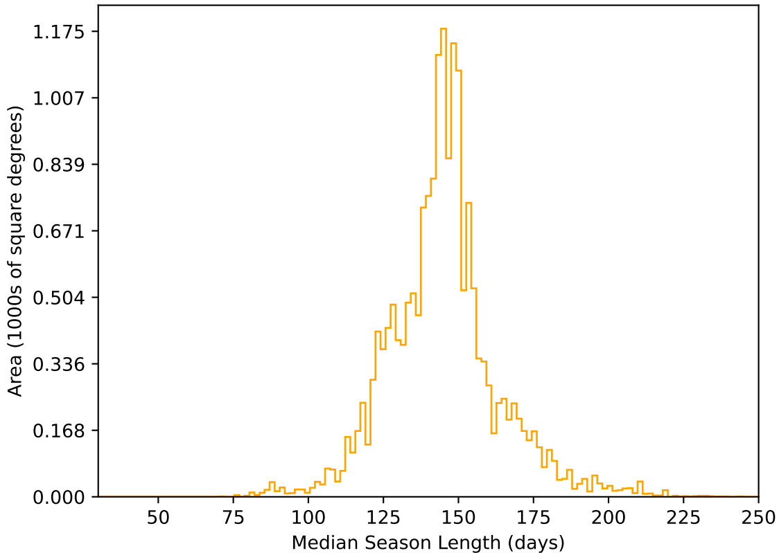
too_elab_r32_d2_gz_v3.4_10yrs WFD r band: Median Season Length
