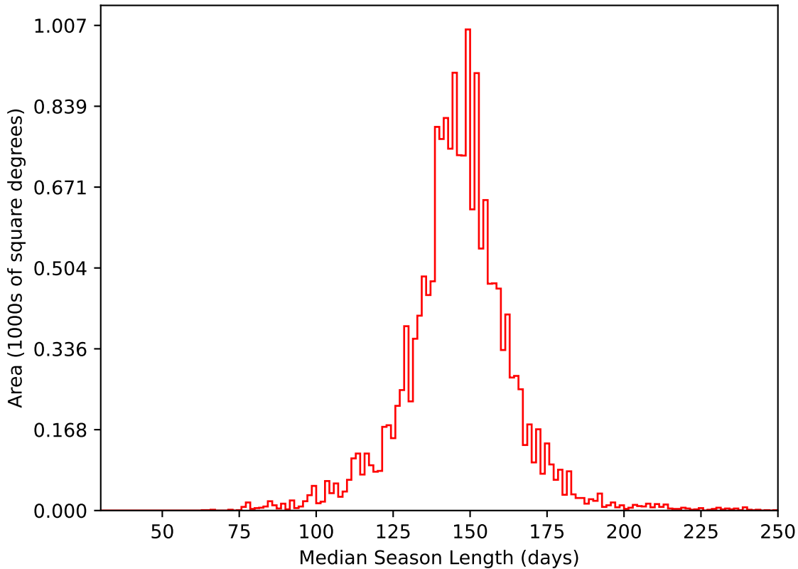
too_elab_r32_d2_gz_v3.4_10yrs WFD i band: Median Season Length
