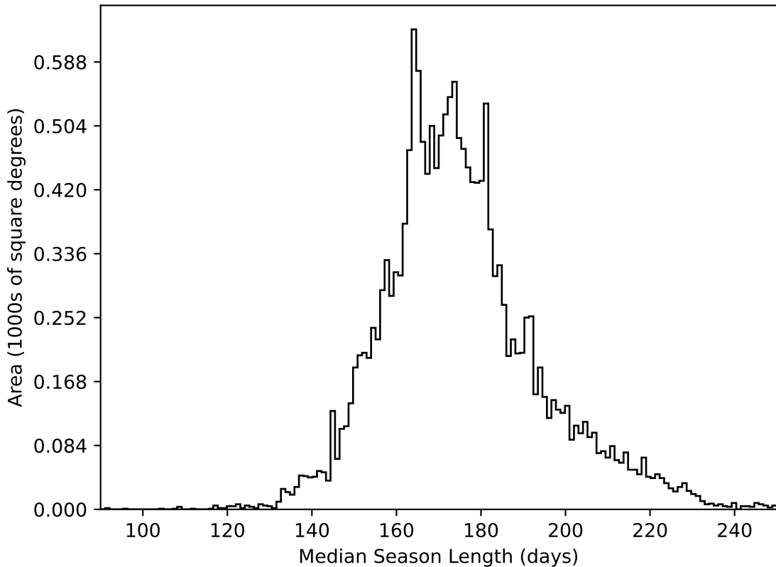
too_elab_r32_d2_gz_v3.4_10yrs WFD all bands: Median Season Length
