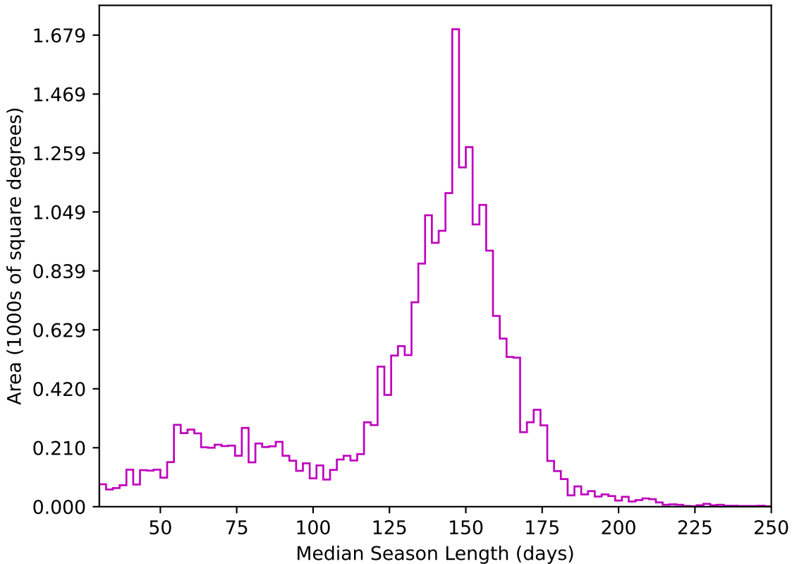
too_elab_r32_d2_gz_v3.4_10yrs All sky z band: Median Season Length
