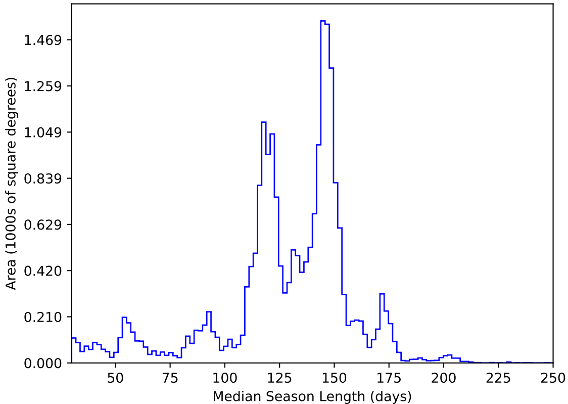
too_elab_r32_d2_gz_v3.4_10yrs All sky y band: Median Season Length
