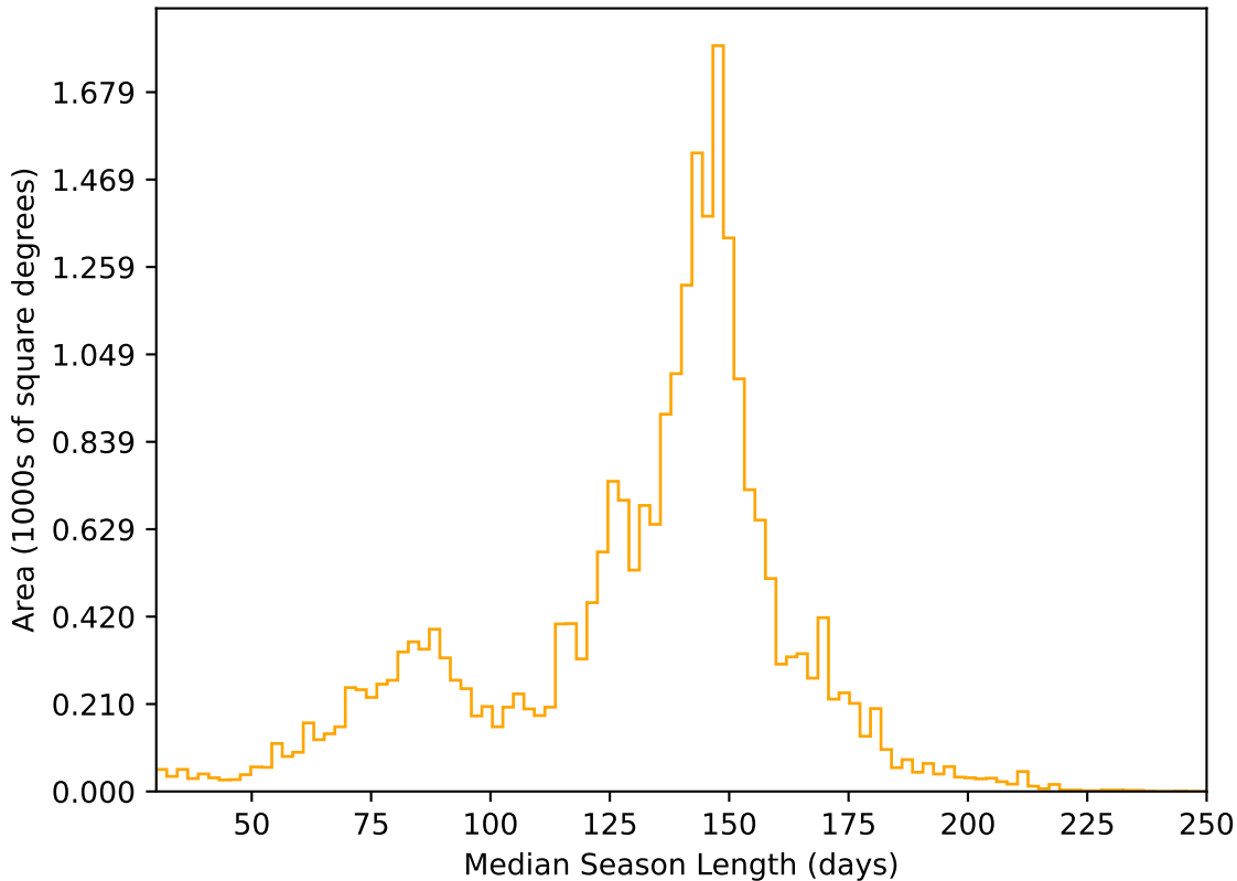
too_elab_r32_d2_gz_v3.4_10yrs All sky r band: Median Season Length
