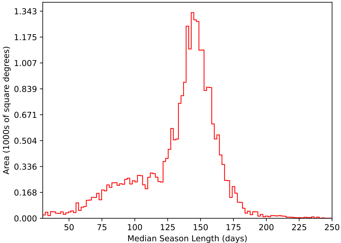
too_elab_r32_d2_gz_v3.4_10yrs All sky i band: Median Season Length
