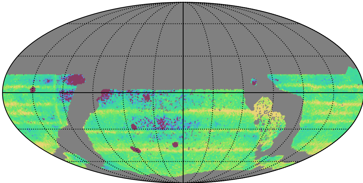
too_elab_r32_d2_gz_v3.4_10yrs WFD: Median Intra-Night Gap
