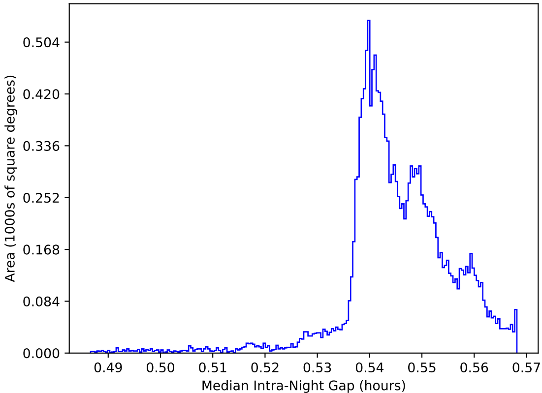
too_elab_r32_d2_gz_v3.4_10yrs WFD: Median Intra-Night Gap
