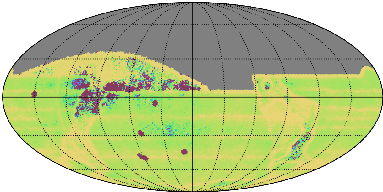
too_elab_r32_d2_gz_v3.4_10yrs All sky: Median Intra-Night Gap
