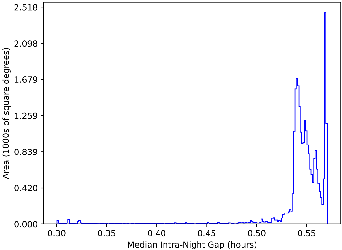
too_elab_r32_d2_gz_v3.4_10yrs All sky: Median Intra-Night Gap
