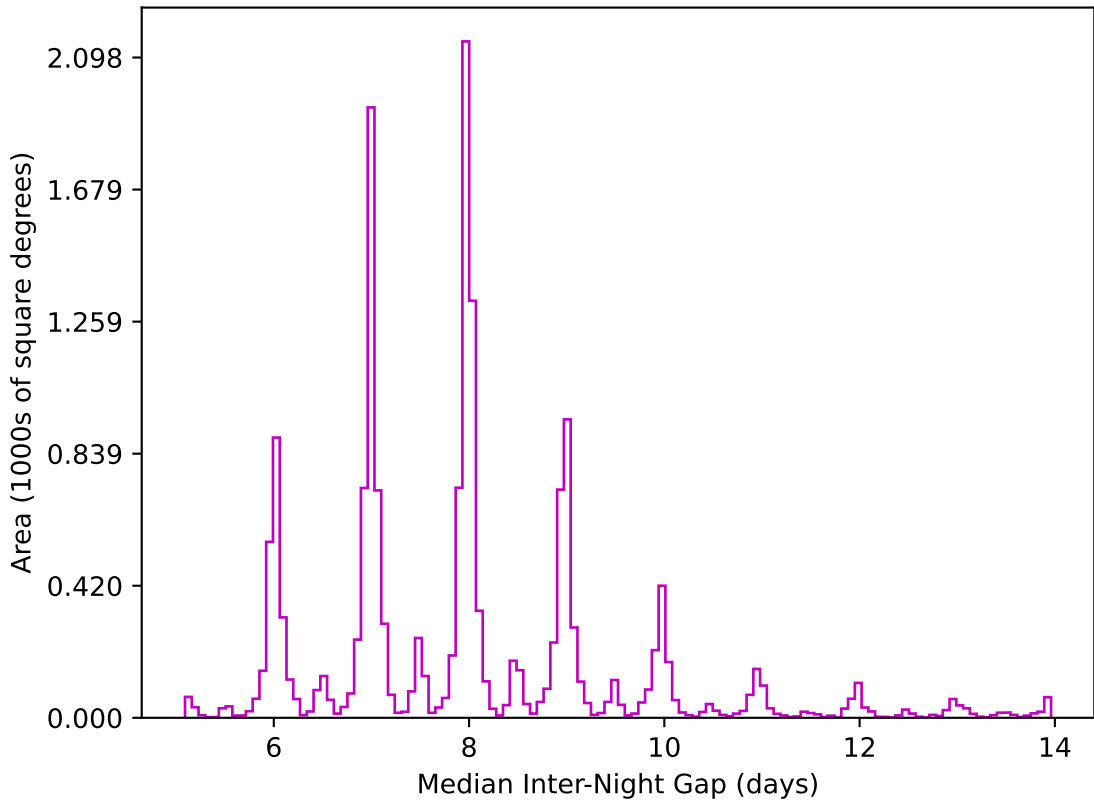
too_elab_r32_d2_gz_v3.4_10yrs WFD z band: Median Inter-Night Gap
