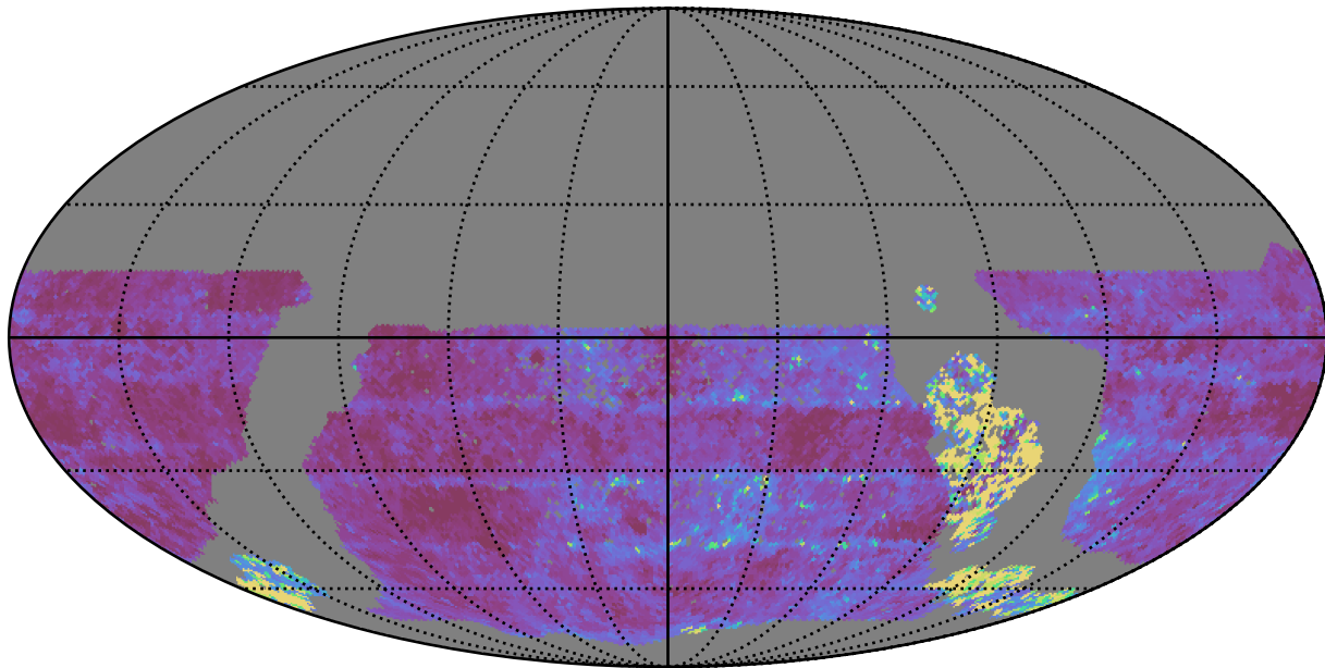
too_elab_r32_d2_gz_v3.4_10yrs WFD u band: Median Inter-Night Gap
