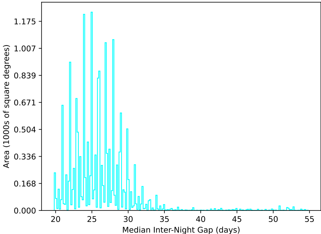
too_elab_r32_d2_gz_v3.4_10yrs WFD u band: Median Inter-Night Gap
