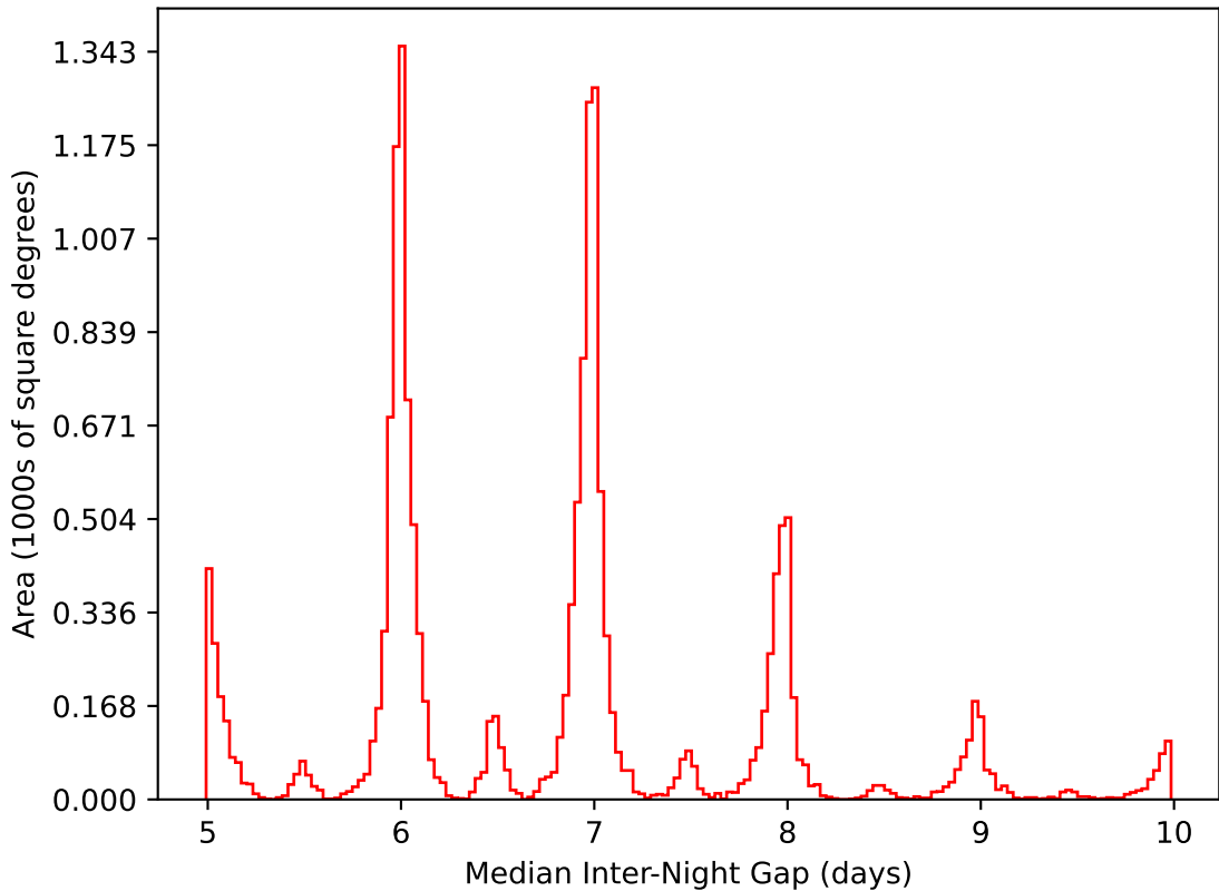
too_elab_r32_d2_gz_v3.4_10yrs WFD i band: Median Inter-Night Gap
