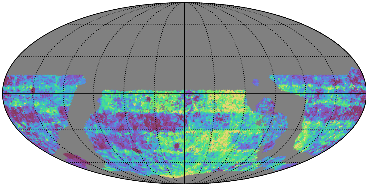
too_elab_r32_d2_gz_v3.4_10yrs WFD g band: Median Inter-Night Gap
