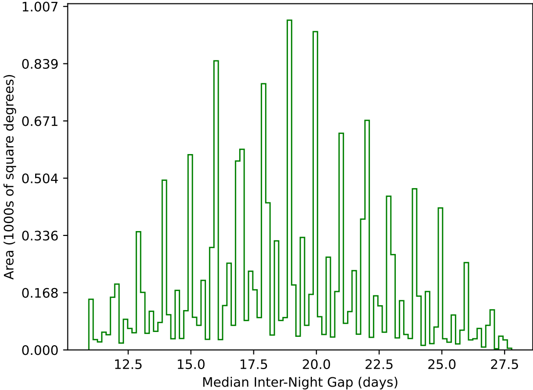
too_elab_r32_d2_gz_v3.4_10yrs WFD g band: Median Inter-Night Gap
