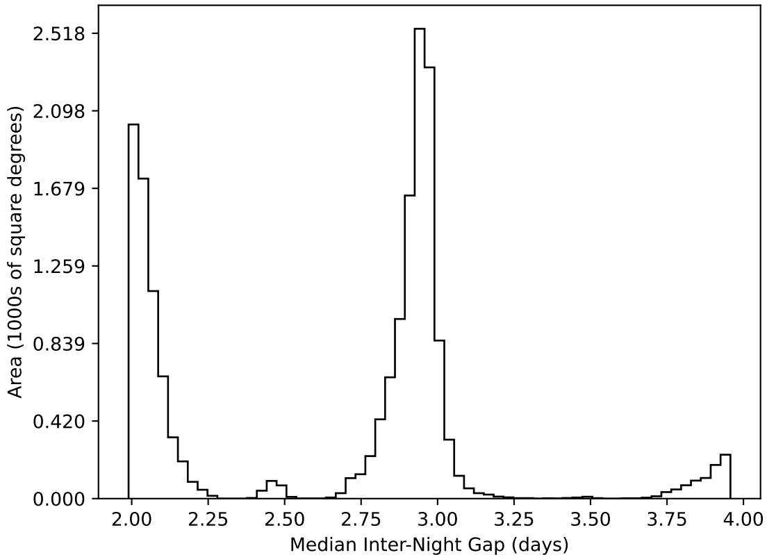
too_elab_r32_d2_gz_v3.4_10yrs WFD all bands: Median Inter-Night Gap
