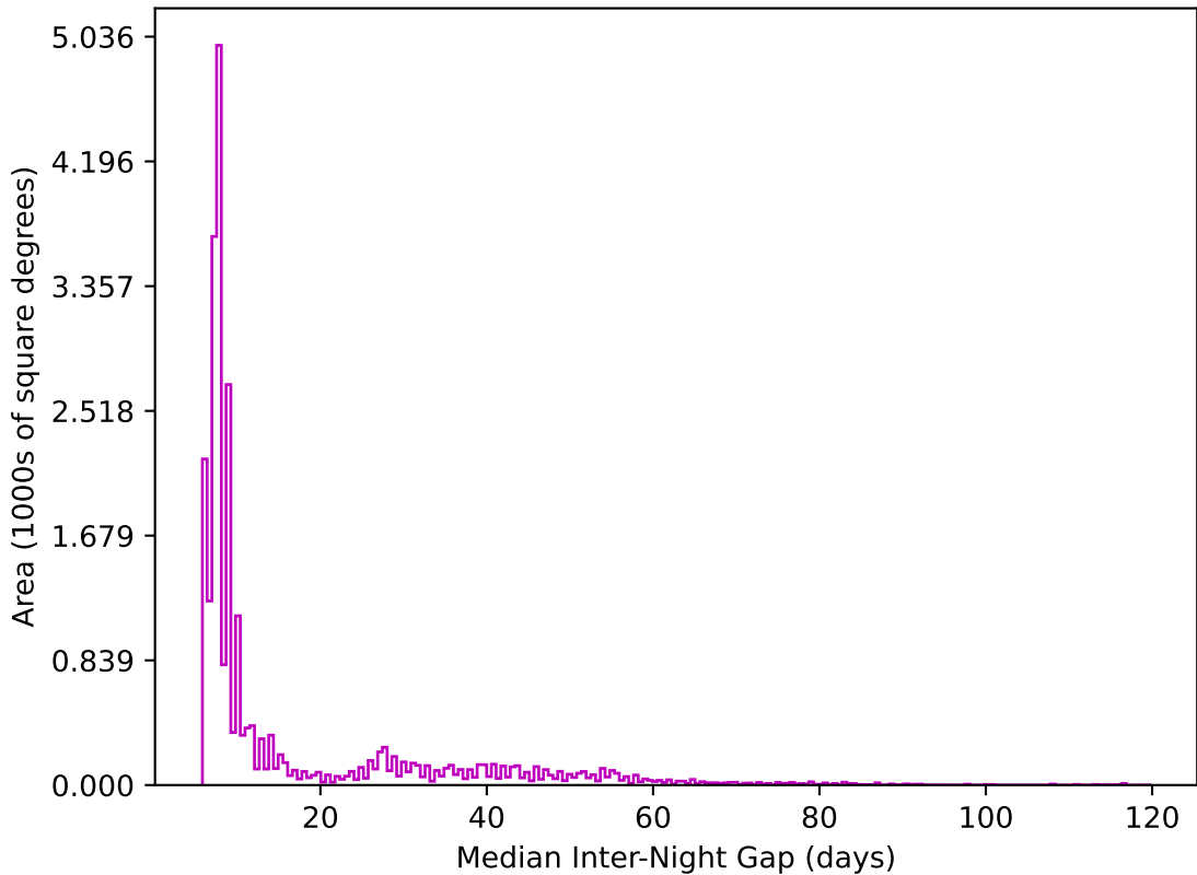
too_elab_r32_d2_gz_v3.4_10yrs All sky z band: Median Inter-Night Gap
