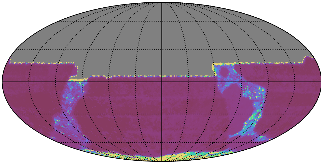
too_elab_r32_d2_gz_v3.4_10yrs All sky y band: Median Inter-Night Gap
