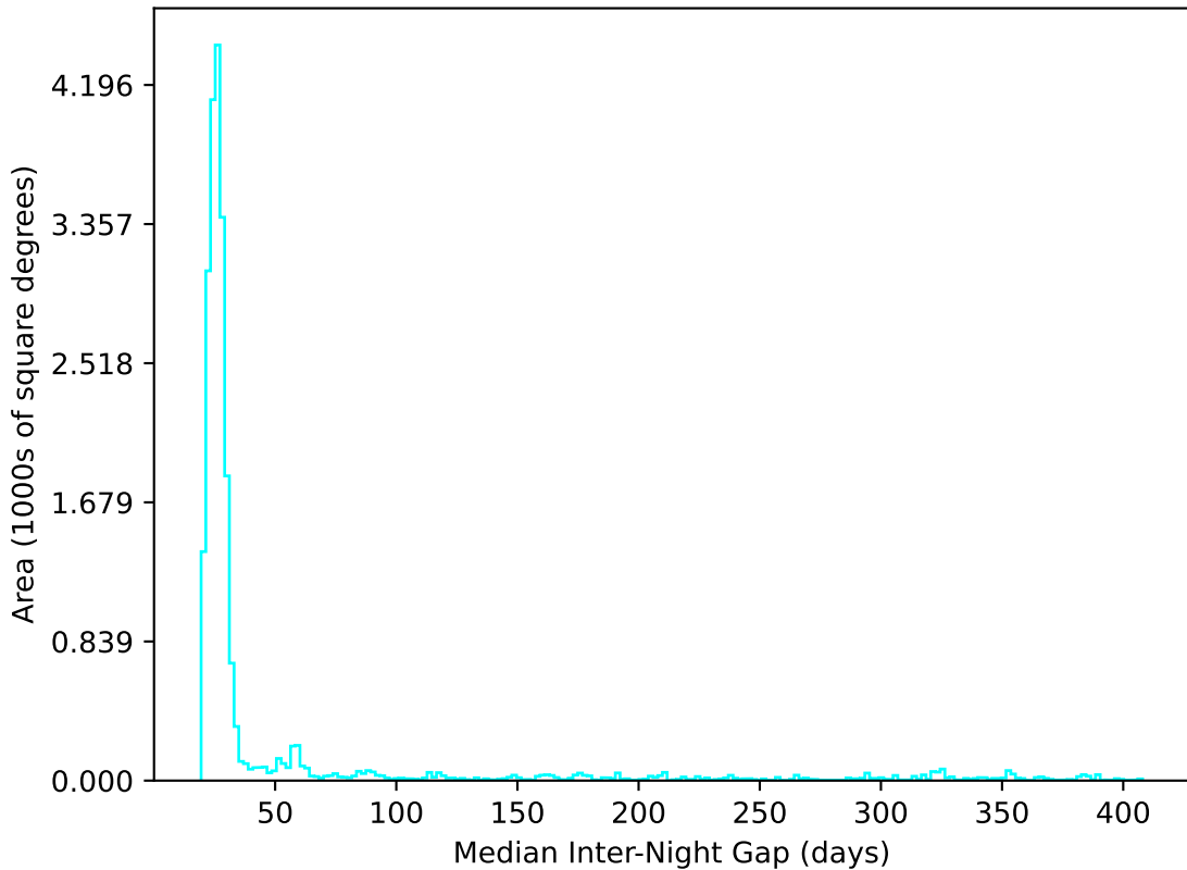
too_elab_r32_d2_gz_v3.4_10yrs All sky u band: Median Inter-Night Gap
