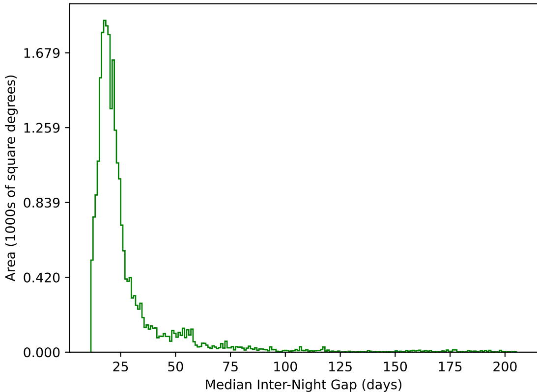
too_elab_r32_d2_gz_v3.4_10yrs All sky g band: Median Inter-Night Gap
