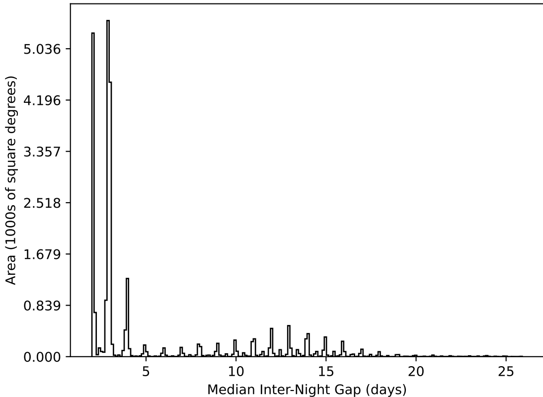
too_elab_r32_d2_gz_v3.4_10yrs All sky all bands: Median Inter-Night Gap
