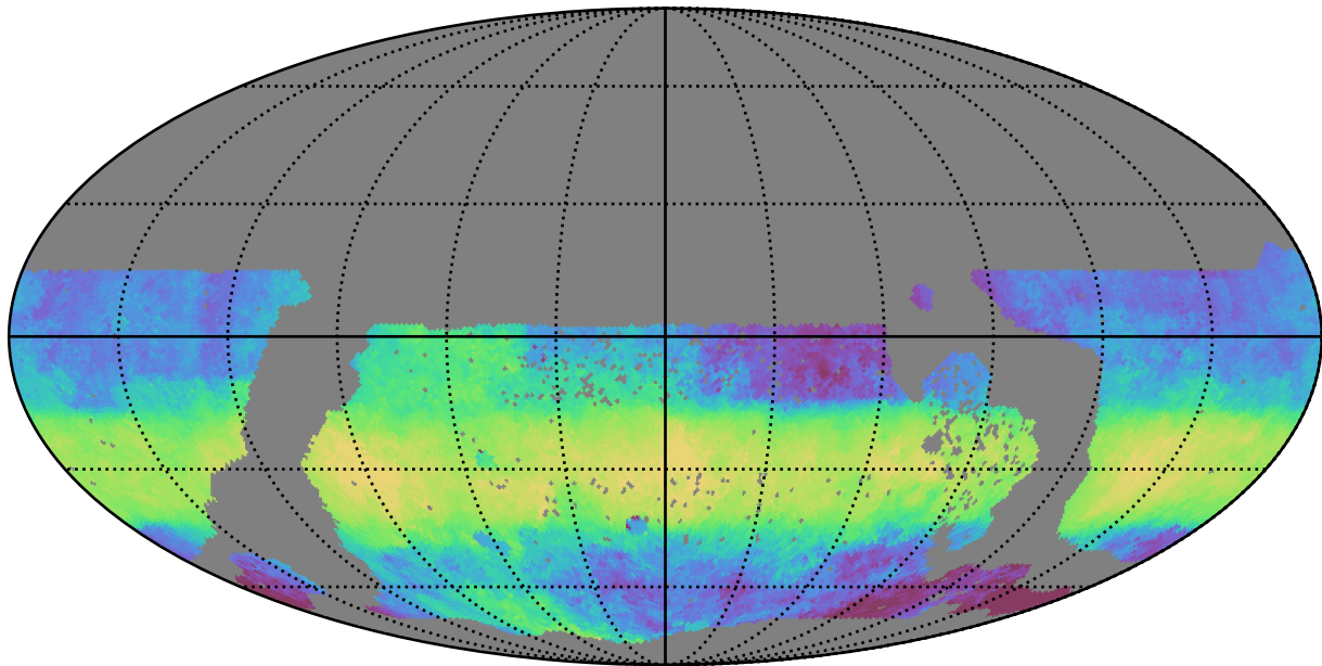
too_elab_r32_d2_gz_v3.4_10yrs WFD z band: Median HA
