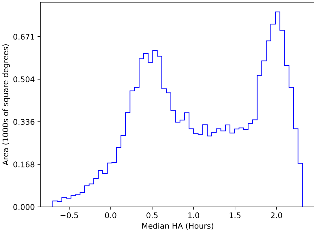
too_elab_r32_d2_gz_v3.4_10yrs WFD z band: Median HA
