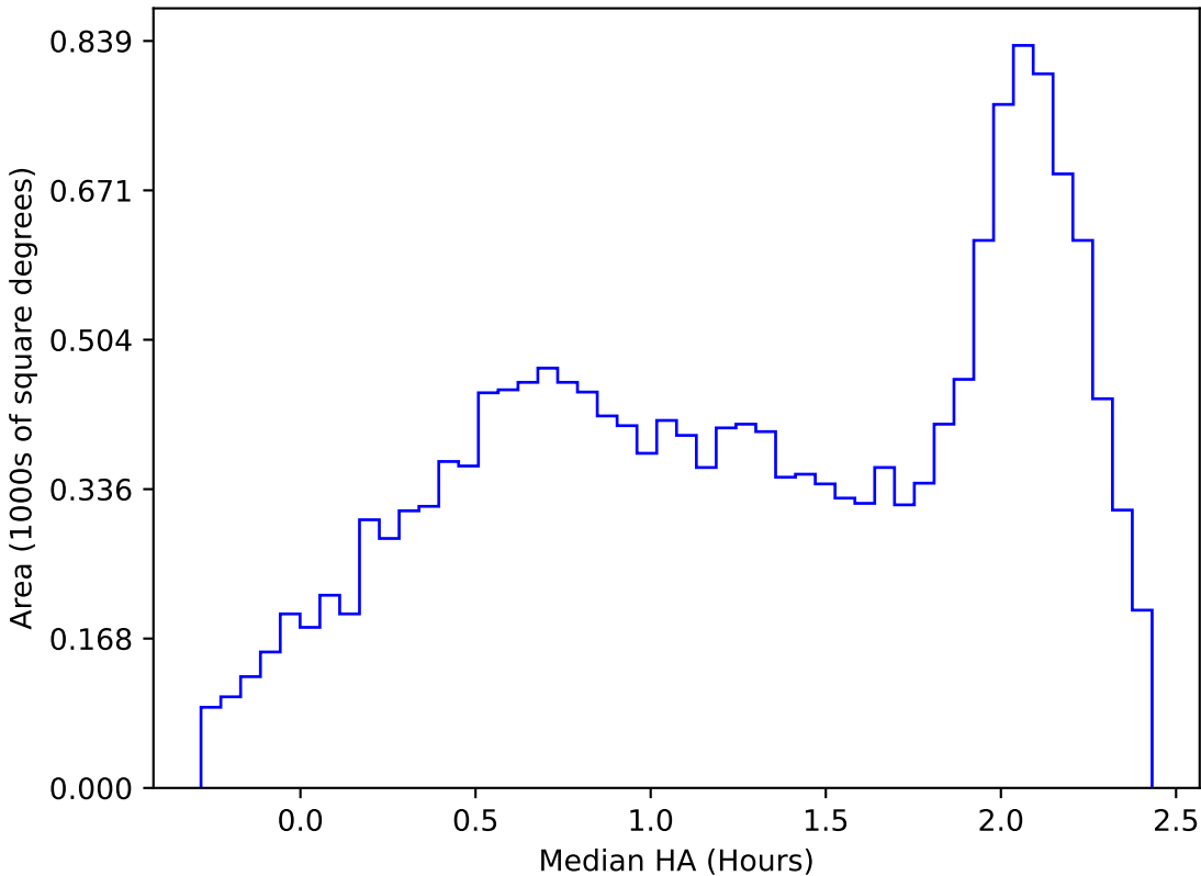
too_elab_r32_d2_gz_v3.4_10yrs WFD y band: Median HA
