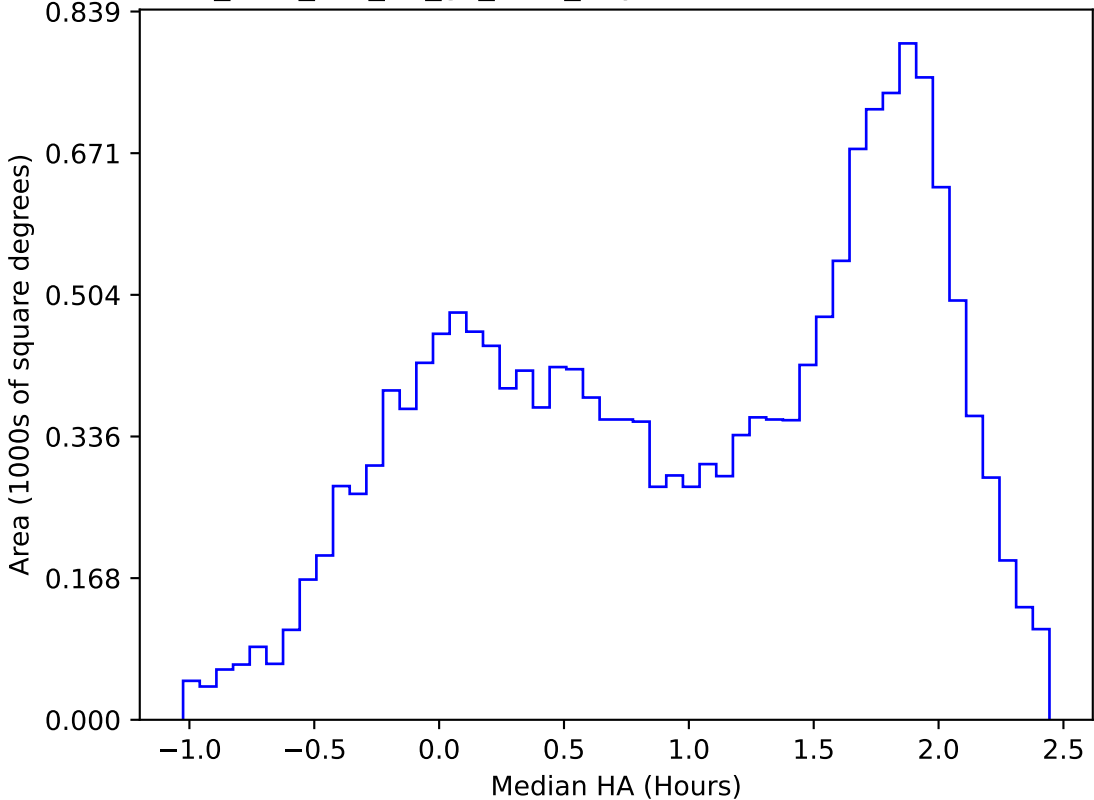
too_elab_r32_d2_gz_v3.4_10yrs WFD u band: Median HA
