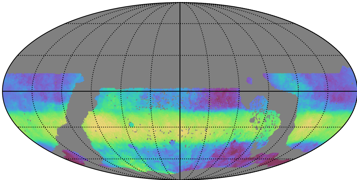
too_elab_r32_d2_gz_v3.4_10yrs WFD r band: Median HA
