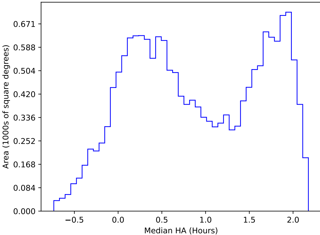
too_elab_r32_d2_gz_v3.4_10yrs WFD r band: Median HA
