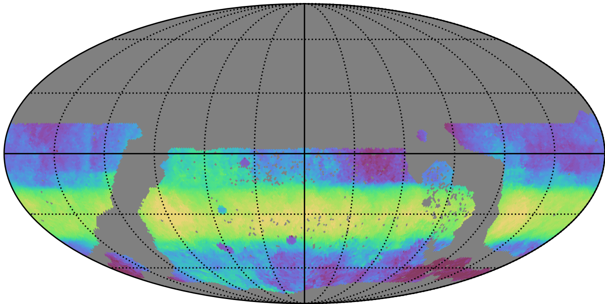
too_elab_r32_d2_gz_v3.4_10yrs WFD i band: Median HA
