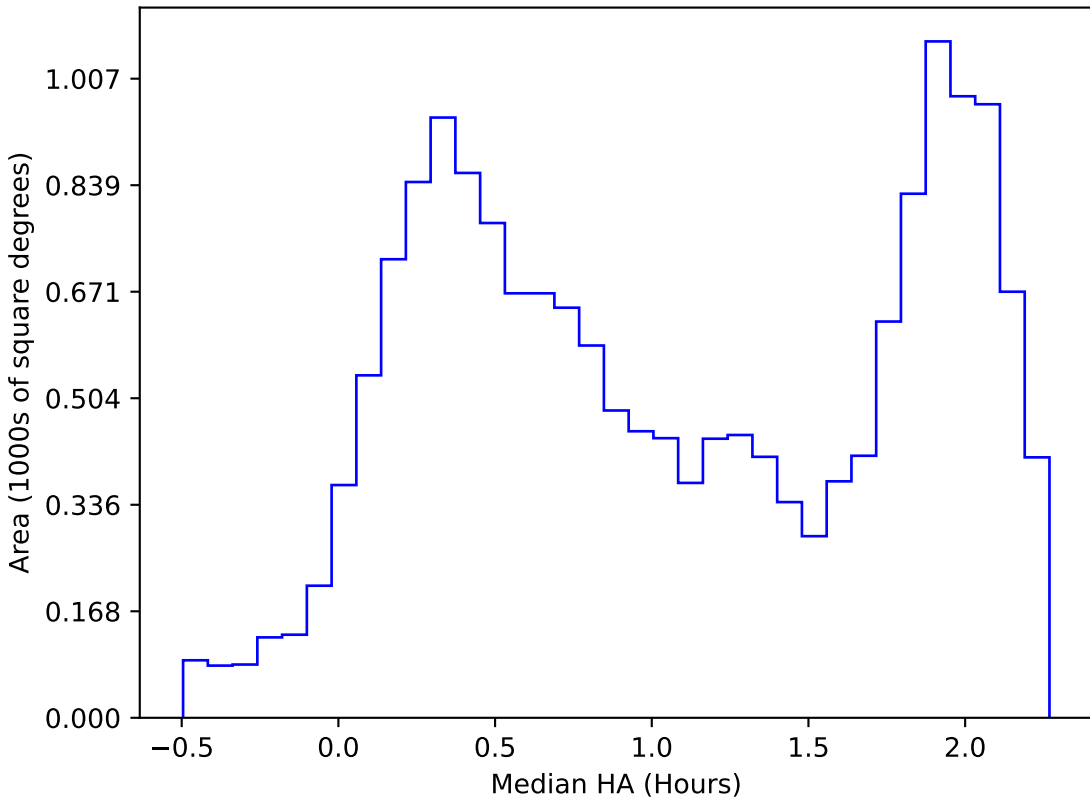
too_elab_r32_d2_gz_v3.4_10yrs WFD i band: Median HA
