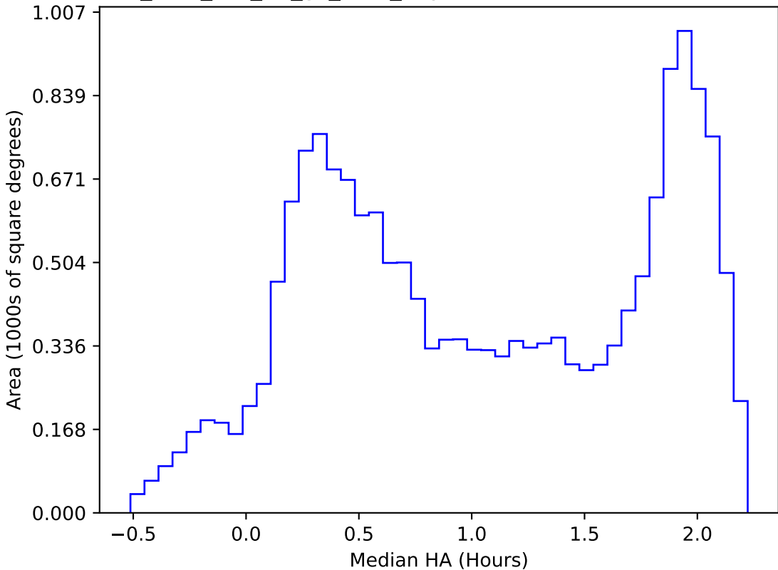
too_elab_r32_d2_gz_v3.4_10yrs WFD all bands: Median HA
